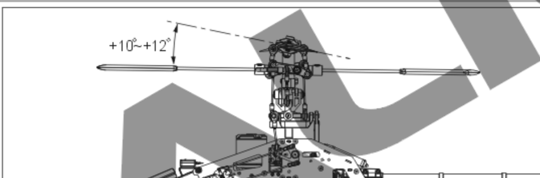
Slick position at high/Throttle 100%/Pitch +10~+12° 搖桿高速/油門100%/Pitch+10~+12°
