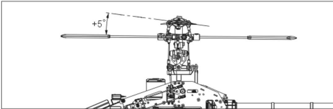
Slick position at Hovering/Throttle 60%/Pitch +5° 搖桿停懸/油門60%/Pitch+5°
