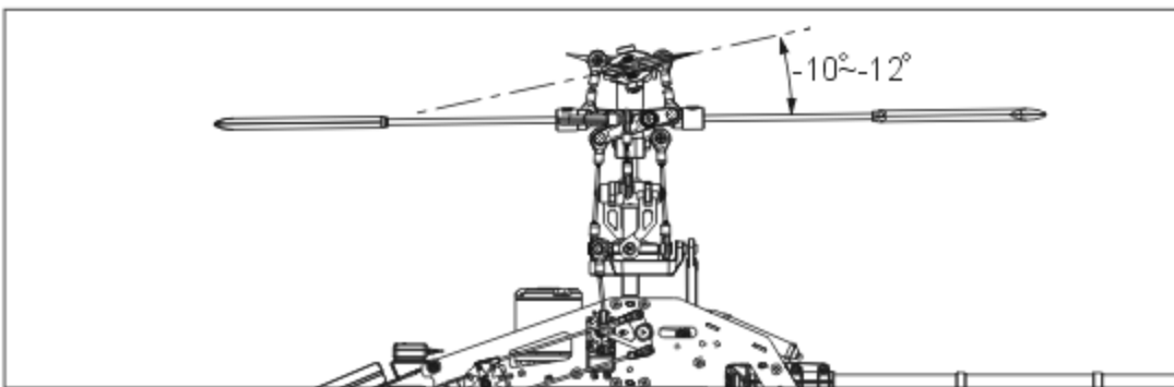
Slick position at low/Throttle 100%/Pitch -10~-12° 搖桿低速/油門100%/Pitch-10~-12°
