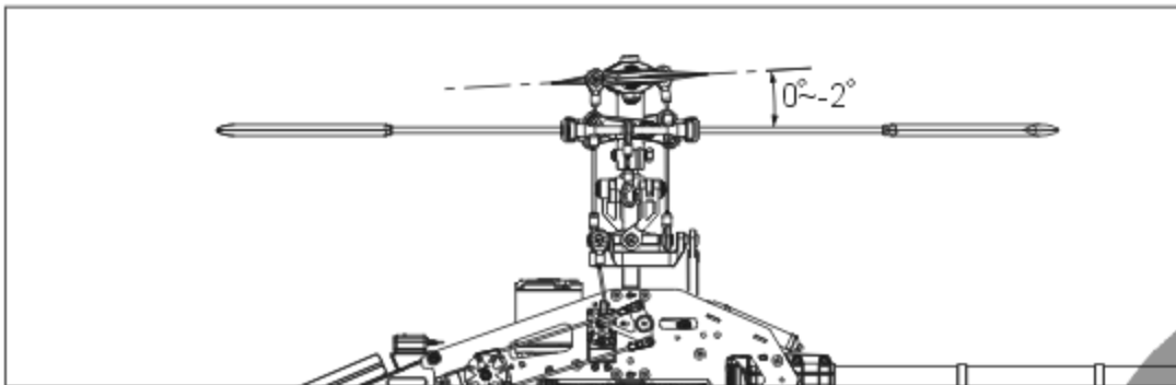
Slick position at low/Throttle 0%/Pitch 0~-2° 搖桿低速/油門0%/Pitch 0~-2°
