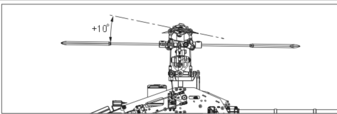
Slick position at high/Throttle 100%/Pitch +10° 搖桿高速/油門100%/Pitch+10°
