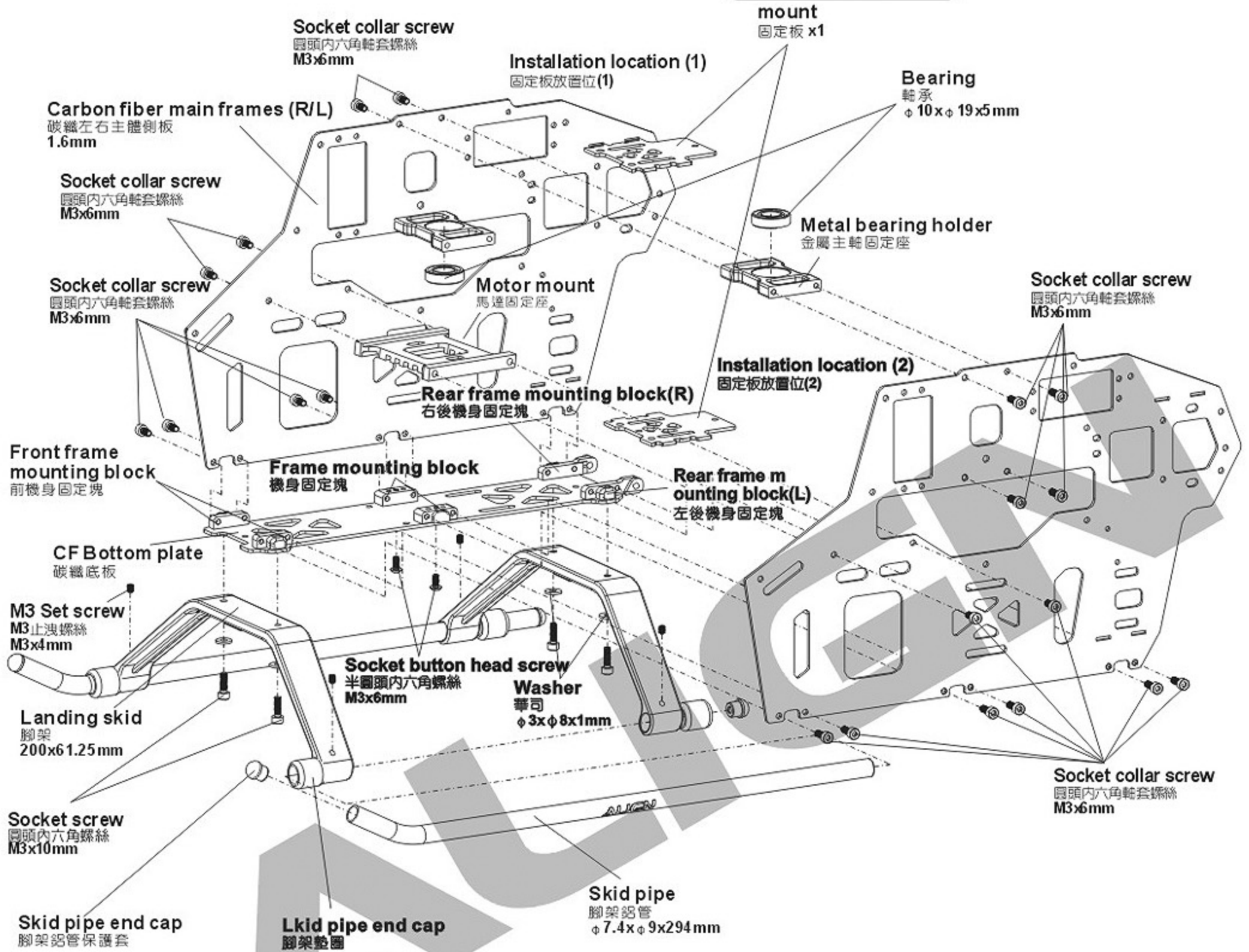
M3 Set screw M3止洩螺絲(M3x4mm) x 4
