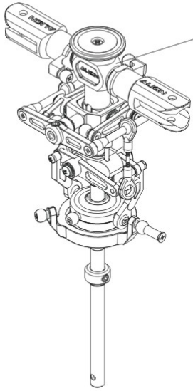
Metal main rotor head assembly 金屬主旋翼組
